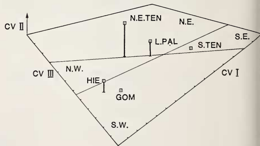
Fig. 2. Three dimensional plot of canonical analysis of male body proportions. The canonical axes (expressing 96% of the variation) are marked in units of within-group standard deviation. N.E. TEN = north-east Tenerife, S. TEN = south Tenerife, GOM = Gomera, HIE = Hierro, L. PAL = La Palma. The geographic origin of the populations are indicated, i.e. north eastern (NE), south eastern (SE), north western (NW) and south western (SW).
